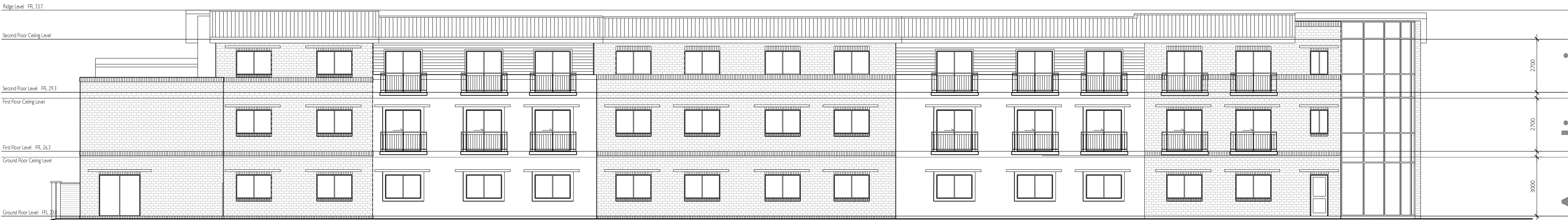
2 East Elevation
